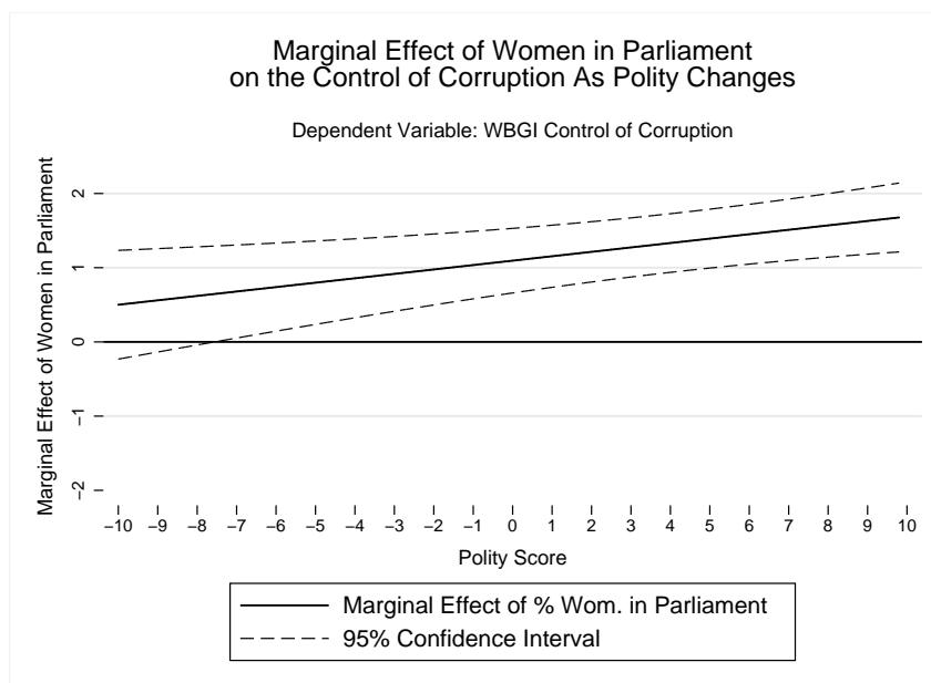
Figure 3: Female Participation in Government and Government Cleanliness, by Polity Score
